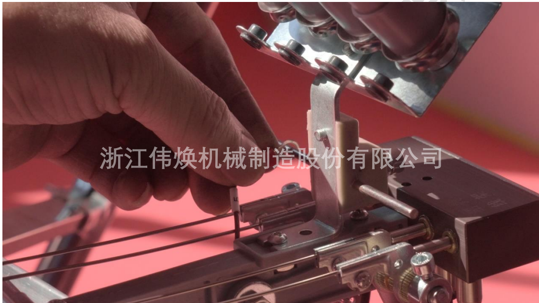
5 号报警线连接跳头报警杆 warning cable #5 connect to picker
