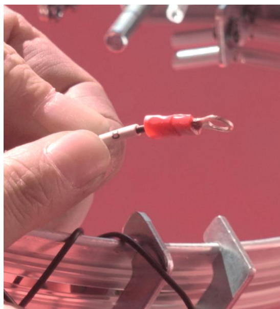
8 号报警线连接上断纱圆圈报警架 warning cable #8 connect to ring holder
