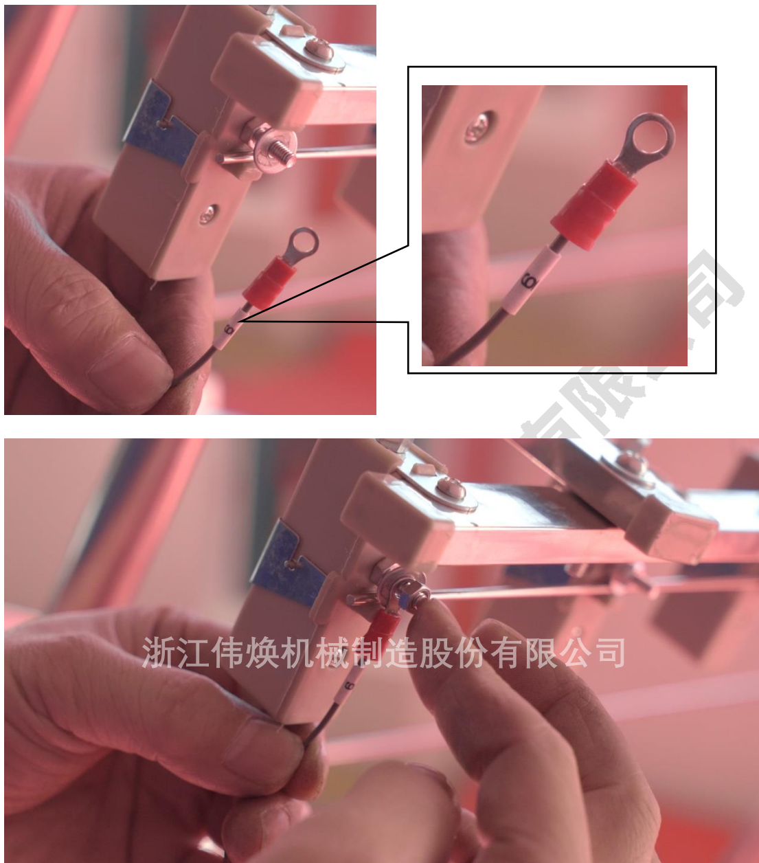
6 号报警线连接紧纱报警架 warning cable #6 connect to yarn tension
